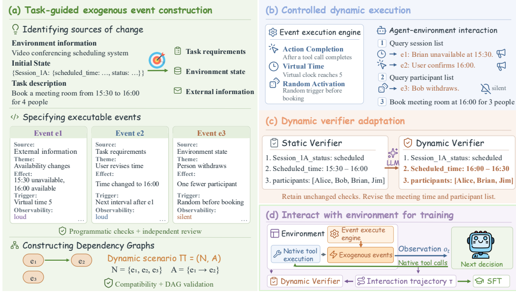
Figure 1: Overview of DynaWeave. (a) The framework generates task-grounded exogenous events from an existing static task, validates their specifications, and organizes compatible events into a dependency graph. (b) An execution engine activates events during agent interaction through action completion, virtual time, or random activation. (c) The dynamic verifier adapts checks affected by realized events while retaining unaffected requirements. (d) Agents interact through the original tools, receiving tool results and permitted event notifications; verified teacher trajectories provide demonstrations for supervised fine-tuning.
