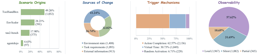
Figure 2: Statistics of the dynamic scenario corpus generated by DynaWeave.
