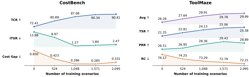
Figure 3: Effect of training scenario quantity on Qwen3.5-4B performance on CostBench (left) and ToolMaze (right). Zero scenarios denotes the baseline Qwen3.5-4B.
