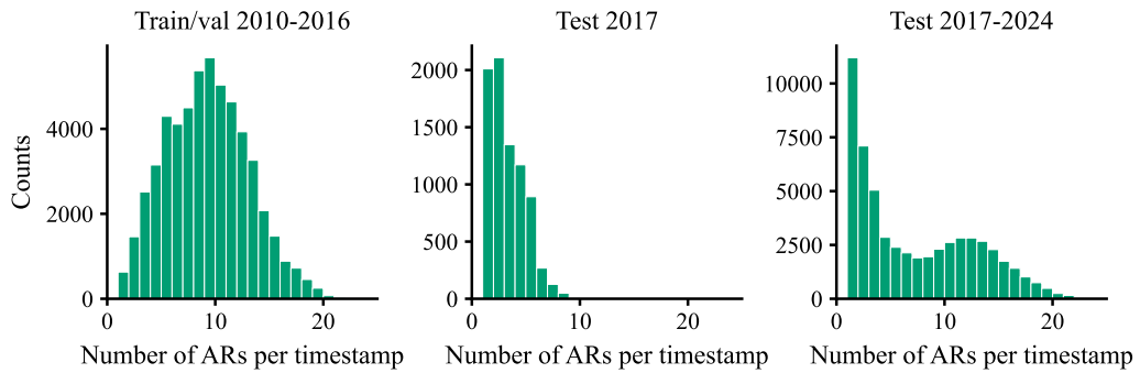
Figure 5: Number of ARs per timestamp across different datasets.
