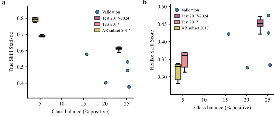
Figure 8: (a) TSS vs. positive-class prevalence: The evaluation subsets with lower positive-class prevalence tend to exhibit higher TSS, with the 2017 and 2017 AR-annotated subsets reaching values of approximately 0.69–0.80, compared with 0.40–0.62 for the other subsets. (b) HSS vs. positive-class prevalence: HSS shows a weaker tendency in the opposite direction, with values of approximately 0.29–0.42 for the highly imbalanced 2017 subsets and approximately 0.45 for the full test set. The validation subsets show no clear monotonic relationship.
