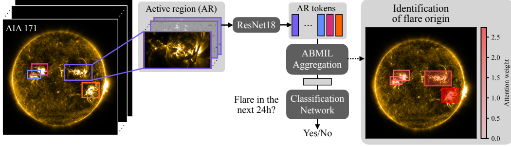
Figure 1: Overview of the ARENA architecture. Each AR across all channels is extracted, rescaled, and provided to a ResNet-18 which compresses the image into a token vector. For one time point, all AR tokens are concatenated and passed through an ABMIL aggregator, resulting in a single summary vector. This vector is processed by a classification head which predicts whether a flare is happening in the next 24 h. At inference, the attention weight can be employed to identify the flare-originating AR.
