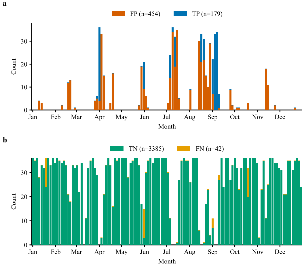
Figure 9: Temporal distribution of the four binary classification outcomes for the 2017 test subset. True positives and false positives are shown among the predicted-positive observations, while true negatives and false negatives constitute the predicted-negative observations. False positives frequently occur in temporal proximity to true positives.
