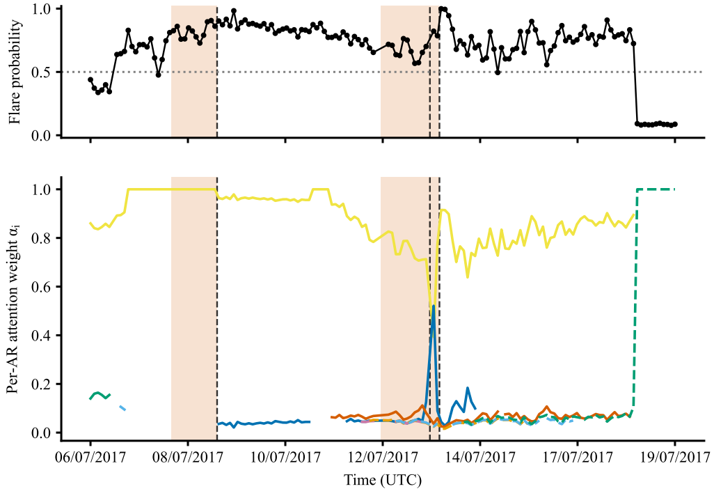
Figure 10: Temporal evolution of ARENA’s predicted M+ flare probability (top) and attention weights assigned to individual active regions (bottom) for July 6th–19th, 2017. The orange shading indicates observations labeled positive according to our flare catalog because an M+ flare occurs within the subsequent 24-hour prediction window. Flares are represented by the black vertical dashed lines. The same active region receives high attention weights \alpha_i across multiple consecutive observations surrounding the two flare events, while the predicted flare probability remains elevated over an extended period. As soon as this region disappears on July 18th, the output probability of the model drops. The yellow line corresponds to SHARP 7075 which is actually causing the two flares according to [9].
