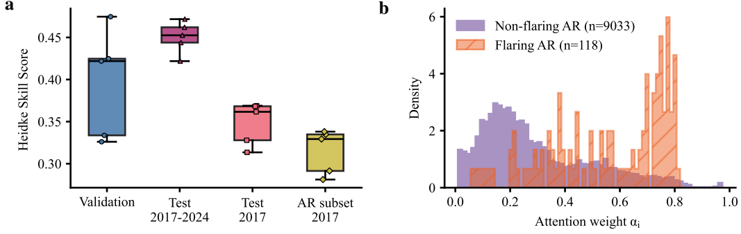
Figure 2: (a) Heidke Skill Score (HSS) across the five temporal cross-validation folds, evaluated on the corresponding validation sets and on three test sets: the full 2017–2024 test period, the 2017 subset, and the 2017 subset containing flares with confirmed AR origins. (b) Density-normalized distribution of attention weights assigned to flare-producing and non-producing ARs for the 2017 subset with confirmed AR origins, using the model with the highest validation HSS among the five cross-validation models.
