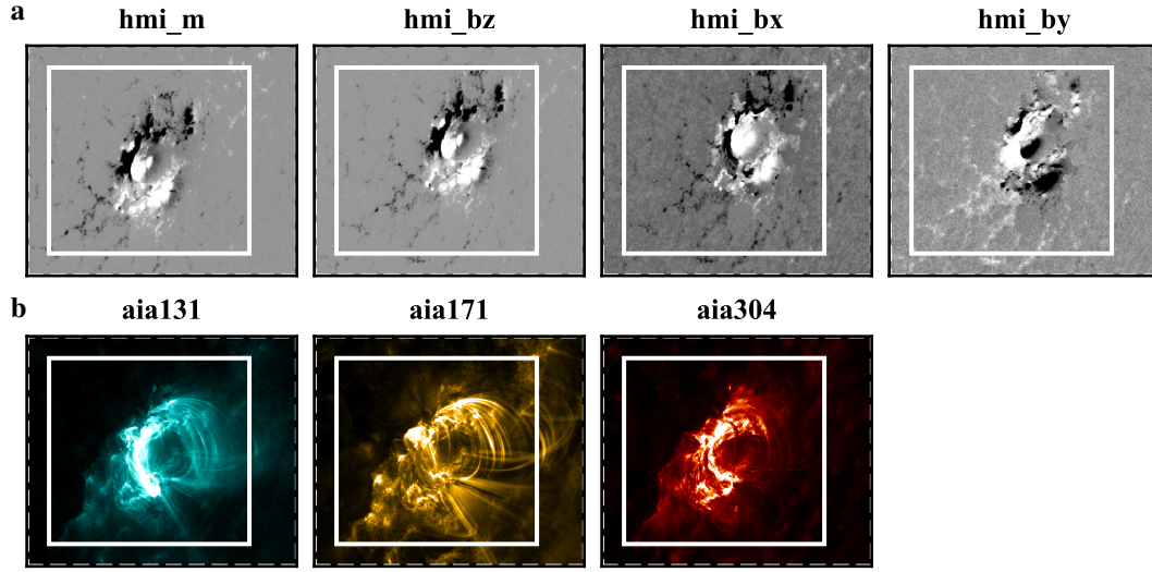
Figure 3: SHARP 7115 cutout image HMI and AIA channels at 2017/09/07 01:00
