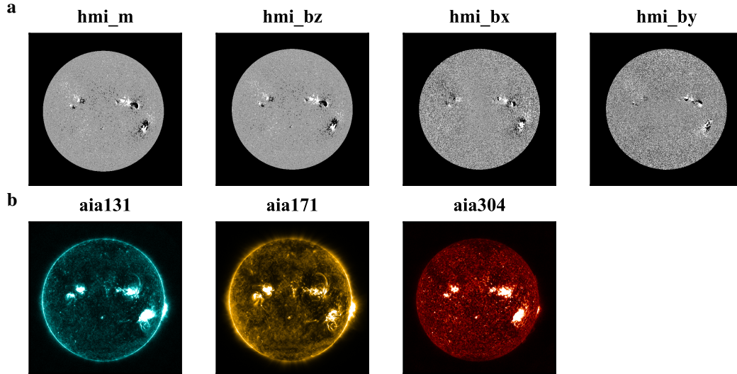
Figure 4: Solar full disk images of four HMI and three AIA channels at 2017/09/07 01:00. hmi_m refers to the line of sight magnetogram.
