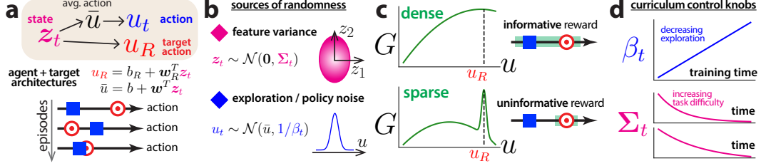
Figure 1: Schematic of task and curriculum learning problem. a) During episode t , the agent receives an F -dimensional state vector z_t as input and must generate a scalar action u_t . The goal of the task is to have u_t match a target action u_R . b) Learning dynamics are stochastic because of feature variance and policy noise. c) We consider two types of returns: a quadratic dense return, and a sparse return that equals a quadratic plus a Gaussian bump. The latter often provides uninformative reward signals if the Gaussian is sufficiently narrow. d) Specifying a curriculum means specifying how some combination of \beta_t and \Sigma_t change over training. Example schedules shown.
