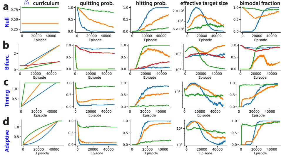
Figure 5: Insights about useful curricula. Each row depicts summaries of simulated REINFORCE trajectories to adjudicate between different types of \beta_t curricula. From left to right: the \beta_t curriculum, quitting probability (likelihood agent is within a fixed small distance from zero), hitting probability (likelihood agent is within \sqrt{v_{\text{eff}}} distance of the target), effective target size v_{\text{eff}} , and the fraction of runs in the bimodal regime. a) Null curricula often do not work, or converge slowly. b) Curricula which involve bifurcations tend to be more effective than ones that do not when the risk of quitting is substantial. The green line produces bifurcating dynamics, while the others do not. c) The timing of the bifurcation matters. If the bifurcation is too early (green), the effective target size remains high and the hitting probability remains low. d) Nonlinear ‘adaptive’ schedules (blue) can outperform linear ones. See Appendix E for a similar plot for \Sigma_t .
