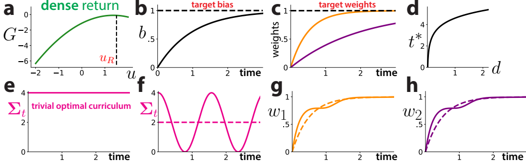
Figure 2: Learning dynamics given dense rewards is simple and complex curricula are unnecessary. a) The dense return is parabolic and has a maximum at u_* := (g/(\alpha + g))u_R . b) Example bias learning trajectory; note that it approaches the optimal bias exponentially quickly. c) Example weight learning trajectories; weights associated with more variable features (orange) converge more quickly than weights associated with less variable features (purple). d) Convergence time scales logarithmically in the discrepancy d := |b_0 - b_*| . e) In the absence of constraints, the optimal curriculum is for feature variances to be as large as possible throughout training. f) With constraints, other solutions (involving potentially non-monotonic changes in task difficulty) are possible. Dashed line: average feature variance over training. g) Weight dynamics with (solid line) and without (dashed line) optimal curriculum. h) Same as in g, but for a weight associated with a different feature. Note that, in the absence of constraints, the optimal curriculum is identical for all feature variances.
