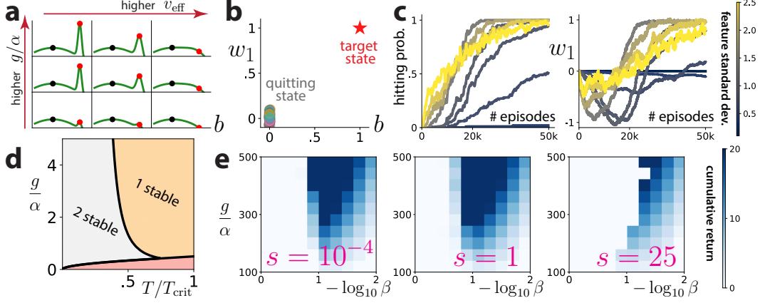
Figure 4: Competing optima produce quitting. a) Visualization of the effective return G_{\text{eff}}(b, w) as a function of b , for different choices of g/\alpha and v_{\text{eff}}(w) . Black dot: location of ‘quitting’ solution, red dot: location of ‘target’ solution. Multiple optima exist when g/\alpha is high and v_{\text{eff}}(w) is low. b) Scatter plot of endpoints of simulated REINFORCE trajectories initialized near zero. They all fail to approach the target state (red star), which is here chosen to be close to 1 for each parameter. c) Left: probability that the agent is within \sqrt{v_{\text{eff}}} of the target parameters over training. Right: the dynamics of the first weight. Different shades of yellow correspond to different feature variances, assuming an isotropic \Sigma = sI . d) Phase diagram of pure bias learning dynamics. e) Heatmap of clipped (between 0 and 20) average cumulative returns of simulated REINFORCE trajectories for different feature variances, assuming \Sigma = sI . Large swaths of parameter space are white, which corresponds to quitting. The moderate feature variance s = 1 performs best.
