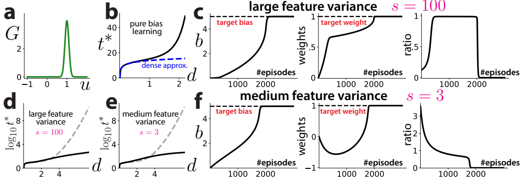
Figure 3: Reward sparsity yields slow learning, and weight dynamics produce an implicit curriculum. a) Return shape assuming no effort term. b) For pure bias learning, the convergence time t^* can be exponentially slow if the scaled distance d := \sqrt{\tilde{\beta}}|b_0 - b_R| is large. c) Example bias and weight learning trajectories in the general case, assuming an isotropic covariance matrix \Sigma = s\mathbf{I} with s = 100 . Rightmost panel: the ratio \frac{(b-b_R)^2}{1/\tilde{\beta} + s\|\mathbf{w} - \mathbf{w}_R\|_2^2} , which transiently remains close to 1. d) Learning with weights converges much more quickly than pure bias learning (dashed gray line) due to an implicit curriculum effect. e) Same as d, but with s = 3 . f) Example bias and weight learning trajectories assuming s = 3 . While the ratio does not as cleanly remain close to 1, convergence behavior is similar. Note that weight dynamics is not monotonic, but involves transient movement away from target weights.
