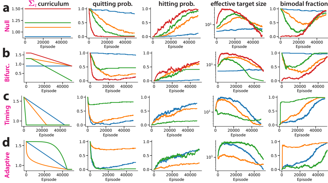
Figure 6: Insights about useful feature variance curricula. Each row depicts summaries of simulated REINFORCE trajectories to adjudicate between different types of \sigma_t curricula. From left to right: the \sigma_t curriculum, quitting probability (likelihood agent is within a fixed small distance from zero), hitting probability (likelihood agent is within \sqrt{v_{\text{eff}}} distance of the target), effective target size v_{\text{eff}} , and the fraction of runs in the bimodal regime. a) Null curricula may not work, although they are more likely to work for \sigma_t than \beta_t . b) Curricula which involve bifurcations tend to be more effective than ones that do not when the risk of quitting is substantial. c) The timing of the bifurcation matters. d) Nonlinear ‘adaptive’ schedules (green) can outperform linear ones.
