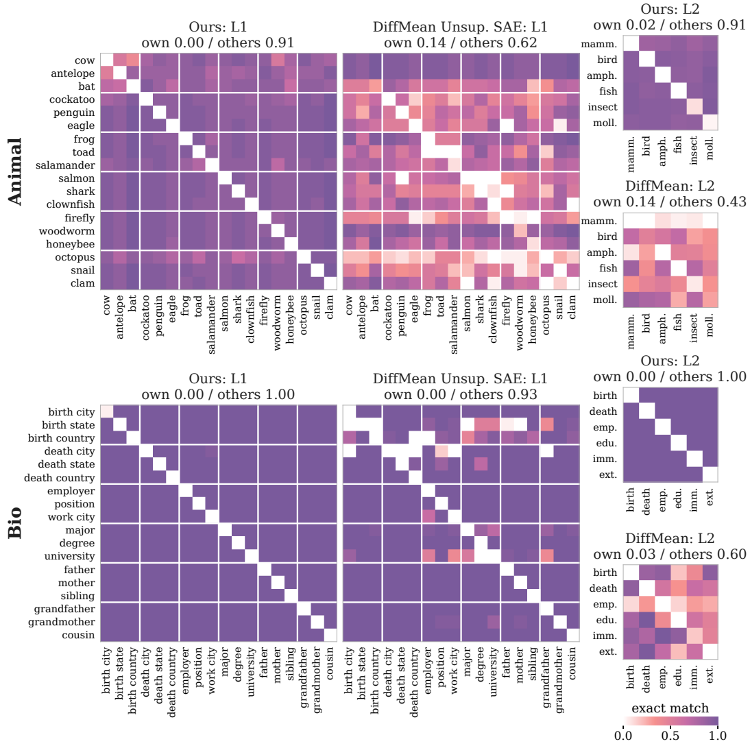
Figure 12: Fig. 6 with concept labels. Row i deactivates the unit of element i ; column j is the exact match on element j .
