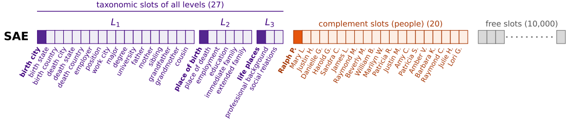
Figure 11: Slot layout of the flat AlignSAE baseline on Bio: a single SAE whose taxonomic slots cover all three levels ( L_1/L_2/L_3 : 18/6/3), followed by complement and free slots. Dark cells mark the slots that the example question should activate. Compare the stacked layout of \mathcal{T}\text{axoSAE} in Fig. 8.
