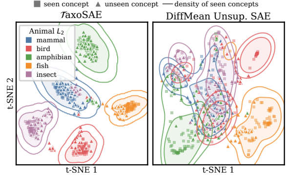
Figure 3: t-SNE of L_2 activations on Animal, colored by L_2 node: squares are trained animals, triangles unseen ones. A triangle inside its color’s contour is placed under the right hypernym. TaxoSAE does this for most unseen animals; DiffMean’s regions overlap. Mollusc is omitted due to heavy overlap in the baseline (App. C).
