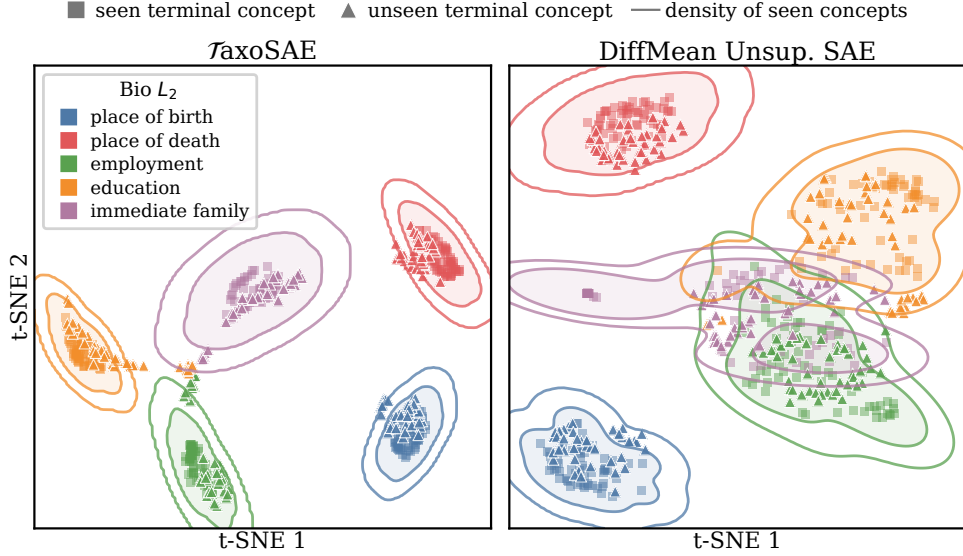
Figure 9: Bio counterpart of Fig. 3: t-SNE of the L_2 readout scores for seen and unseen terminal relations. The extended-family node is omitted for readability; Table 7 includes it.
