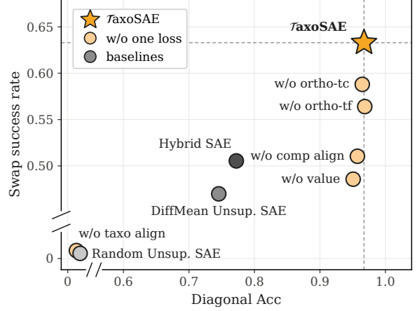
Figure 7: Ablation on Bio (upper right is better). Removing taxonomic alignment collapses both metrics to random; removing others mainly lowers swap success.
