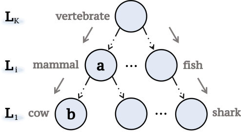
Figure 1: A taxonomy: each edge (a, b) is an is-a link from hypernym a to hyponym b ; dashed edges mark further levels and nodes. Gray labels: a K = 3 example from the Animal taxonomy (full taxonomy in App. A). TaxoSAE uses one SAE per level L_k (Fig. 2).
