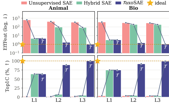
Figure 5: Activation fragmentation (EffFeat) and concentration (Top1C) per taxonomy level on Animal and Bio; dashed lines mark the ideal single unit. \mathcal{T} axoSAE activations are the most concentrated.
