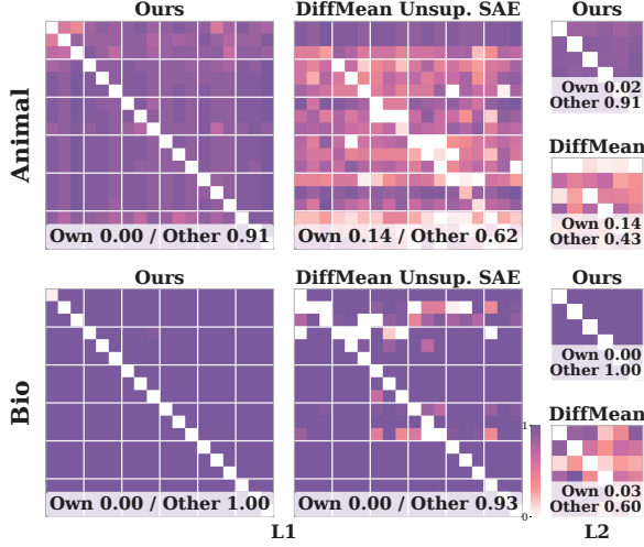
Figure 6: Selectivity on Animal (top) and Bio (bottom): row i deactivates element i 's unit; column j is the exact match on element j . Ideally the diagonal is white and the rest dark, as for \mathcal{T} axoSAE; DiffMean also lightens off-diagonal cells, especially at L_2 . Own ( \downarrow )/Other ( \uparrow ): mean accuracy on target/non-target elements. Labeled version: Fig. 12.
