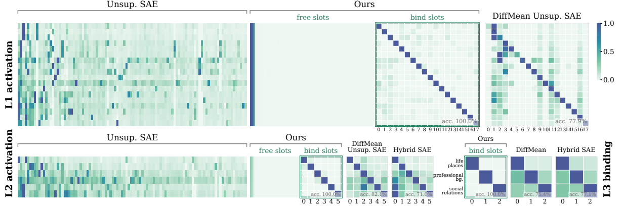
Figure 4: Normalized activations ( L_1/L_2 ) and binding matrices ( L_1-L_3 ) on Bio. Rows group questions by their terminal node and its hypernyms. Wide panels show activations over all units: the unsupervised SAE spreads each concept over many features, while \mathcal{T} axoSAE concentrates it in bind slots. Square panels show each concept’s assigned unit; a diagonal means perfect binding, and “acc.” is the binding accuracy.
