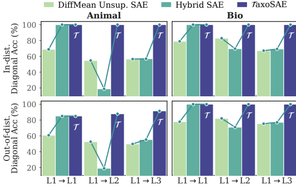
Figure 10: Diagonal accuracy on terminal-level questions read at L_1 – L_3 , with seen templates (ID, top) and unseen rephrasings or synonyms (OOD, bottom). \mathcal{T} axoSAE is best at every level in both settings.
