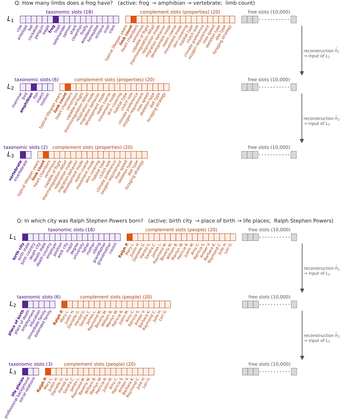
Figure 8: Slot layout of the three stacked SAEs on Animal (top) and Bio (bottom). Each level has one taxonomic slot per node at that level, one complement slot per complementary element, and 10,000 free slots; \text{SAE}_{k+1} reads the reconstruction of \text{SAE}_k . Dark cells mark the slots that the example question should activate: its terminal node and that node’s hypernyms in the taxonomic slots, and its complementary element at every level.
