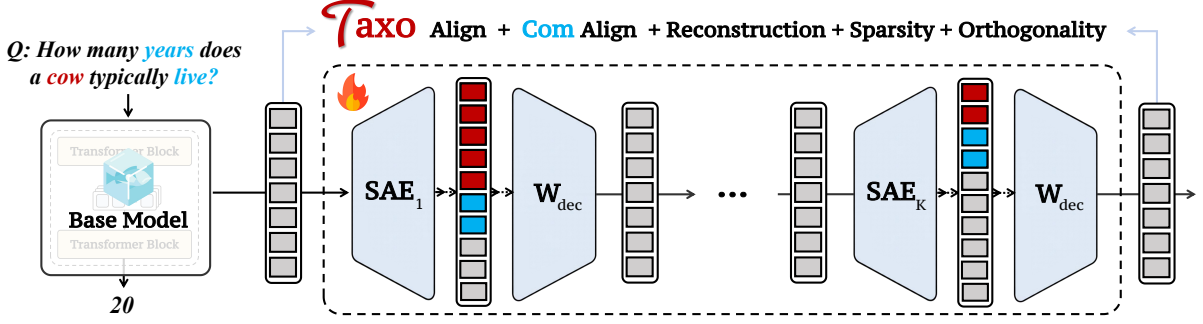
Figure 2: Overview of \mathcal{T} axoSAE. We train stacked SAEs on a frozen LLM’s last-token hidden state. (1) Stacked SAEs : one SAE per taxonomy level ( L_1, \dots, L_K in Fig. 1), each mapping the reconstruction of the level below onto its hypernyms. (2) Taxonomic alignment loss : each taxonomic slot is trained to fire when the input involves its node or any of the node’s hyponyms. Complement slots bind the complementary element; reconstruction, sparsity, and orthogonality losses complete the objective. Figure 8 shows the full slot layout of each level on both taxonomies.
