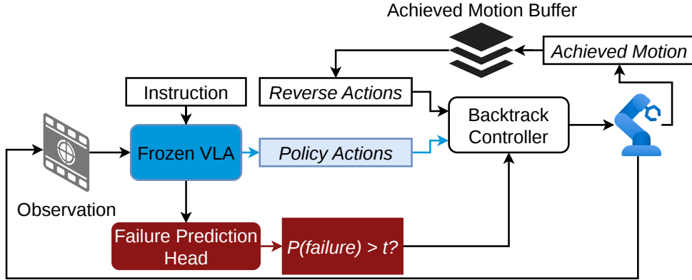
Figure 1: Overview of Backtrack. A small failure prediction head reads features already computed by the frozen VLA and estimates the probability that the current episode will fail. When the predicted failure probability exceeds the threshold t , the Backtrack controller suppresses the policy’s proposed actions and instead retraces recent achieved arm motion stored in a buffer. Otherwise, the policy’s actions are executed normally. The resulting state is observed by the unchanged VLA and the control loop continues. Achieved motion is added to the buffer during normal policy execution; motion executed during backtracking is not. The diagram abstracts over differences in action generation between the evaluated VLAs.
